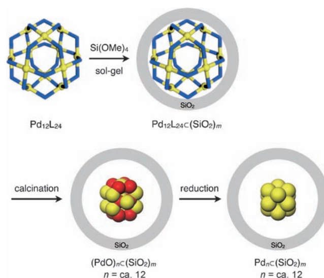
Figure 1. Preparation of (\text{PdO})_n and \text{Pd}_n cluster-incarcerated silica nanoparticles ( n = \text{ca. } 12 ).
